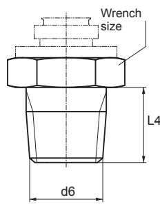
Conical screw threads
